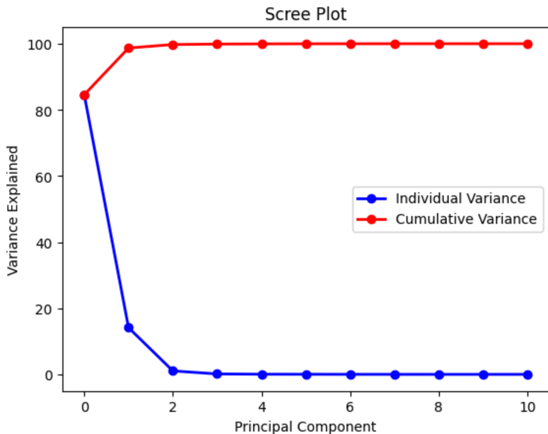
Fig. 5: Scree Plot
