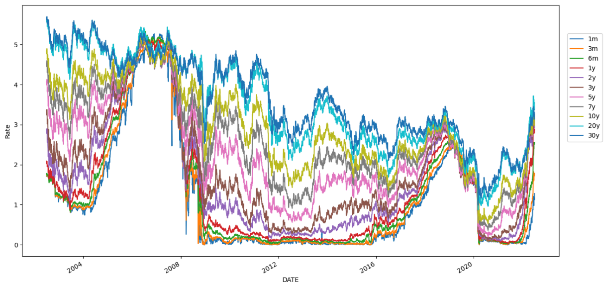
Fig. 1: Yield Curve Movement
