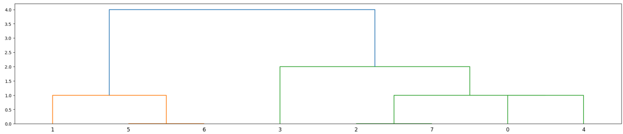
Fig. 1: Dendrogram with Single Linkage
