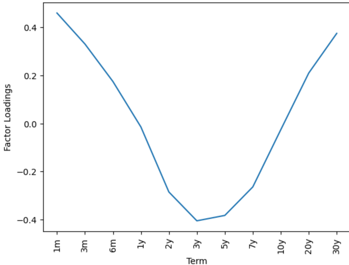
Fig. 4: The Third Factor Loading
