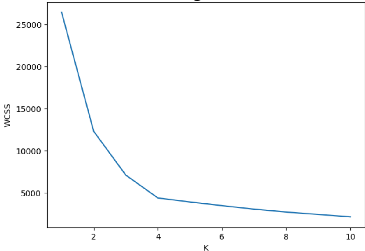
Fig. 6: The Elbow Method K-Means Clustering(The Elbow Method)
