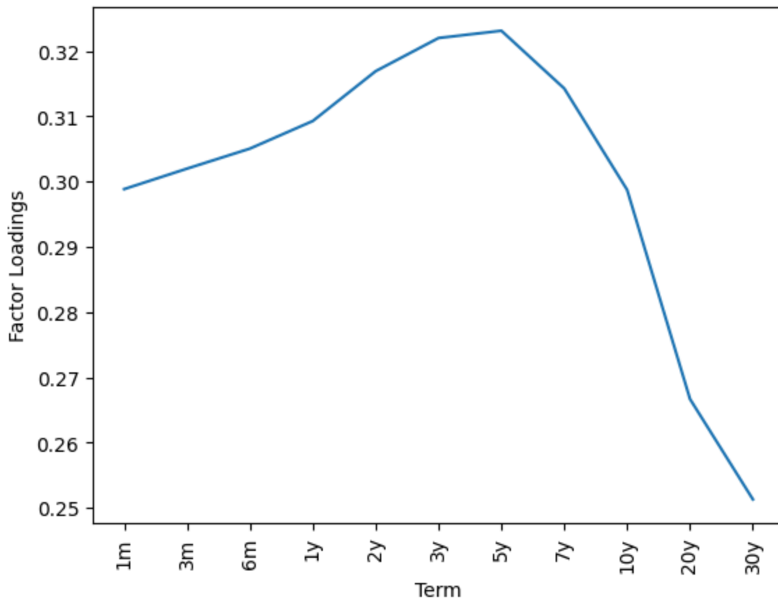
Fig. 2: The First Factor Loading
