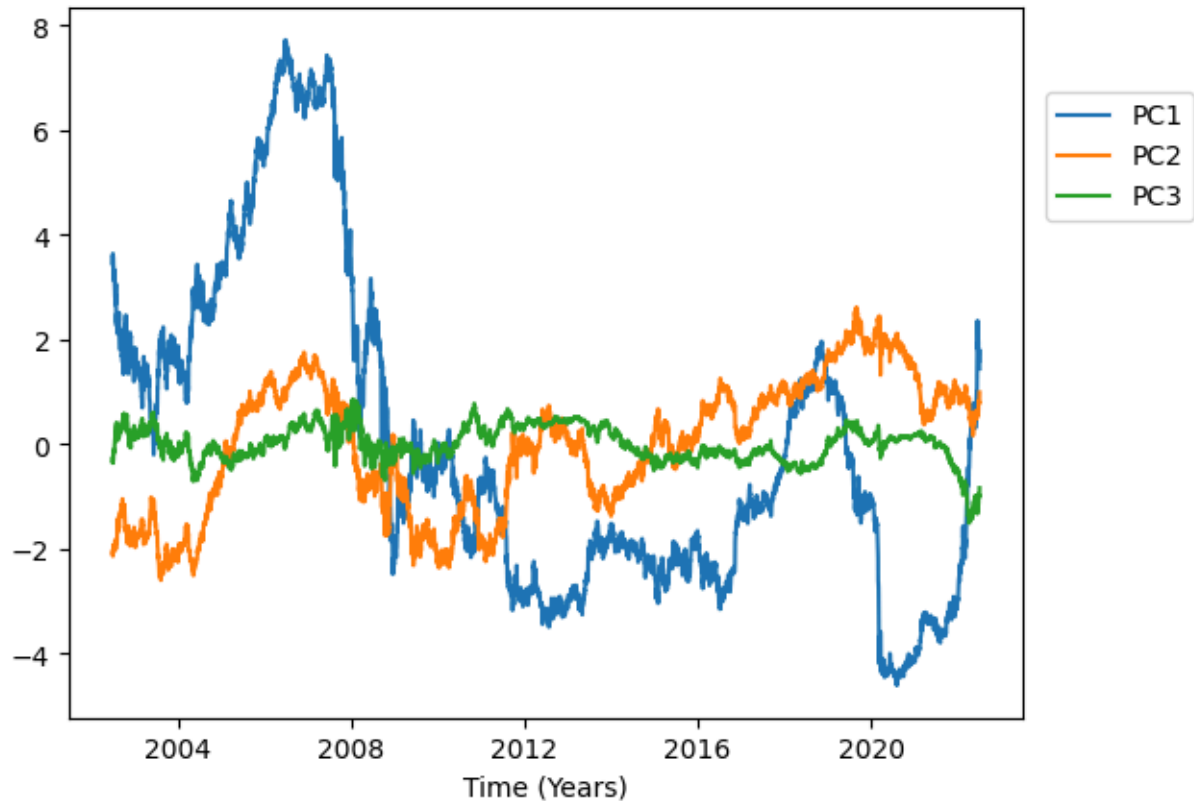
Fig. 6: Principal Component
