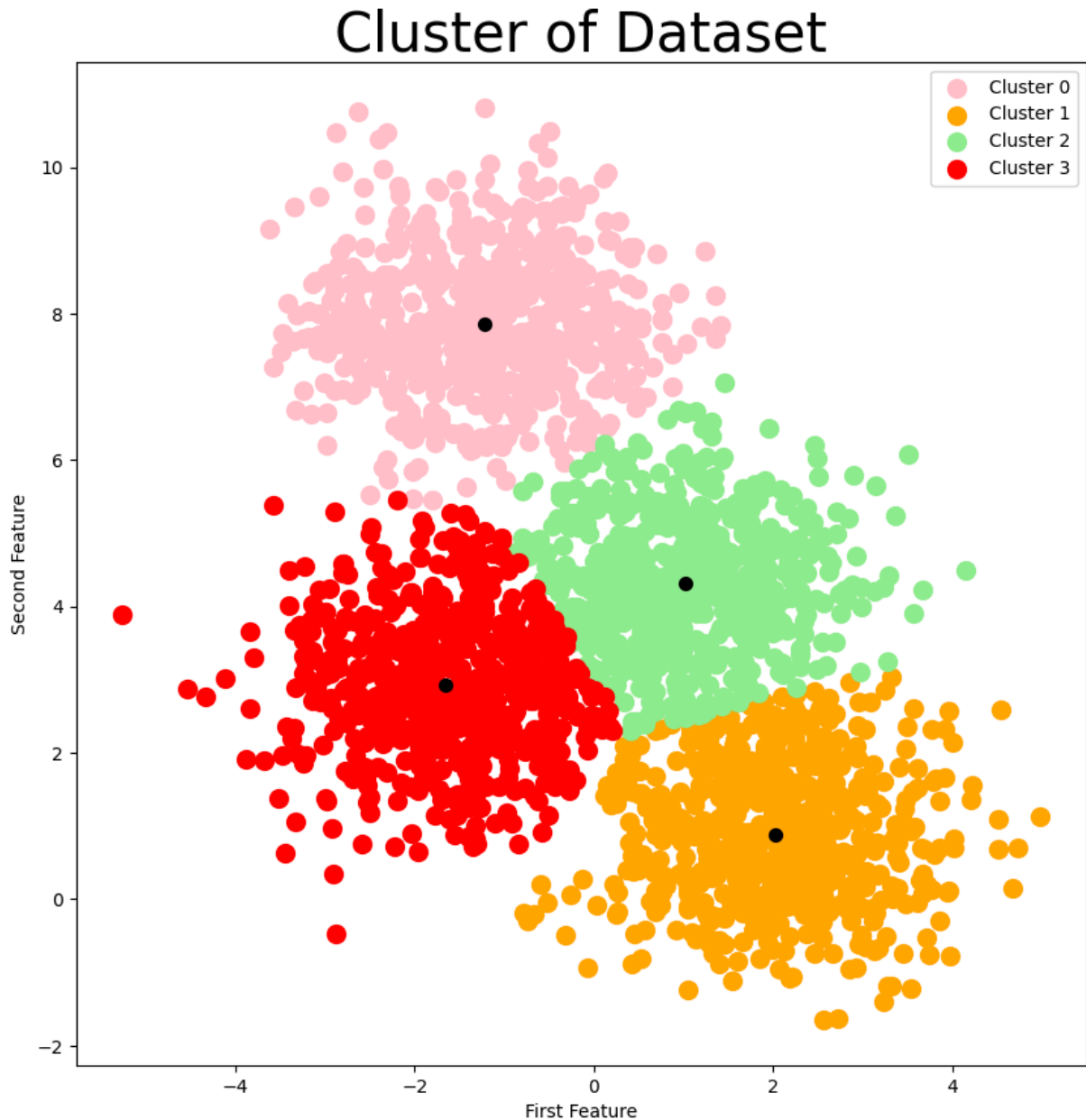
Fig. 7: Clustering Results
