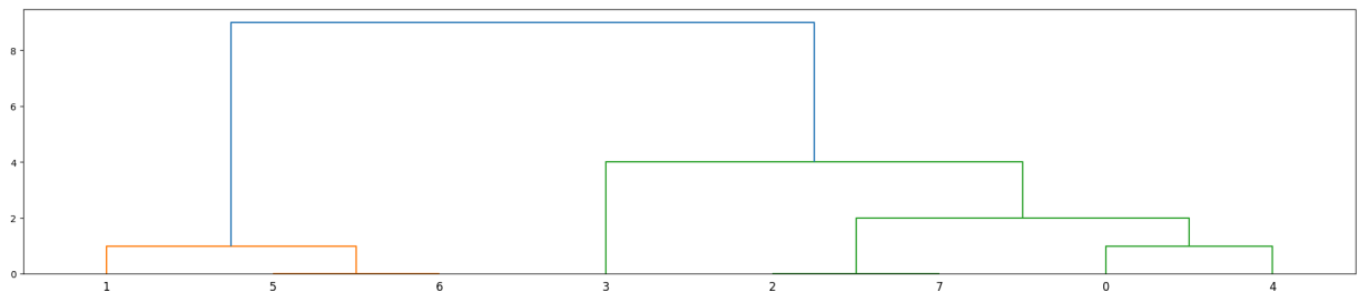
Fig. 2: Dendrogram with Complete Linkage
