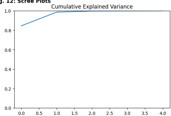
Fig. 12: Scree Plots
