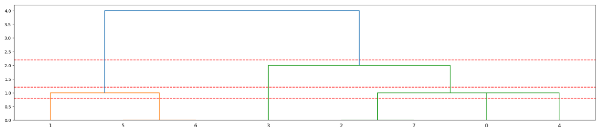
Fig. 6: Dendrogram with Different Horizontal Lines
