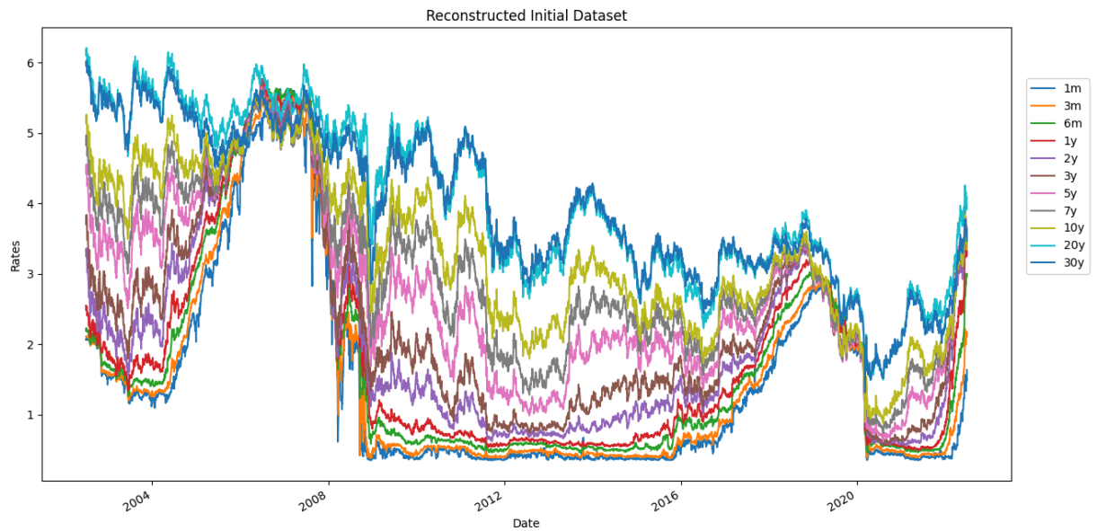
Fig. 9: Reconstructed Initial Dataset
