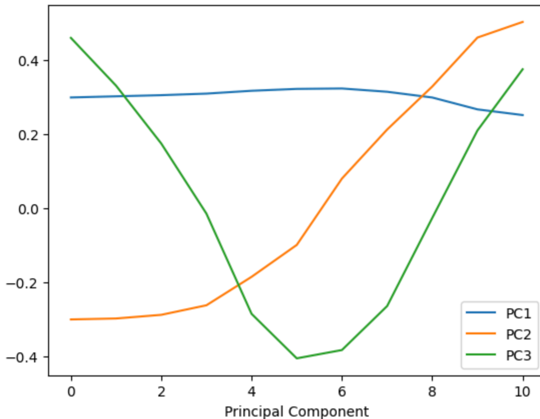
Fig. 13: Factor Loadings
