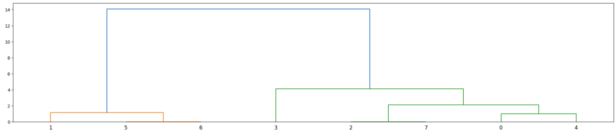
Fig. 5: Dendrogram with Ward Linkage
