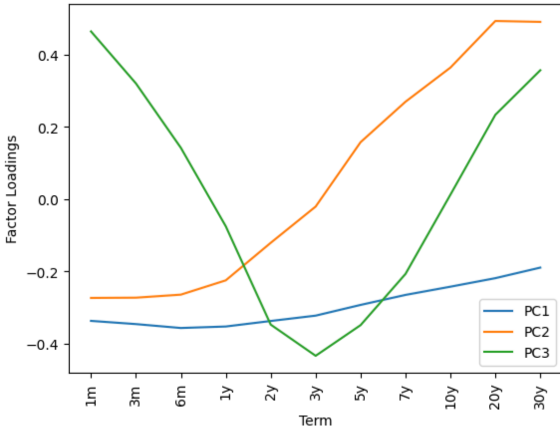
Fig. 7: The Factor Loadings
