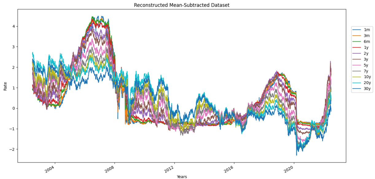
Fig. 8: Reconstructed Mean-Subtracted Dataset
