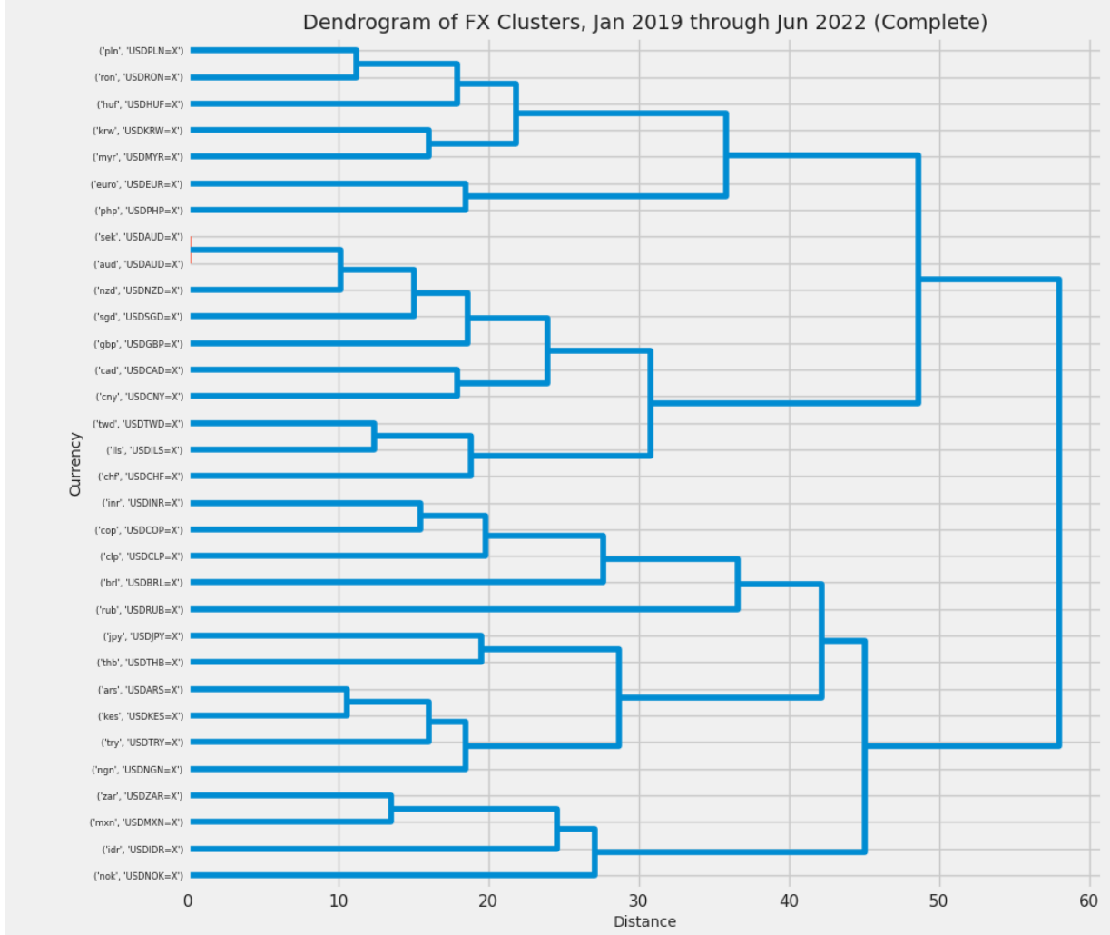
Fig. 12: Dendrogram with Complete Linkage
