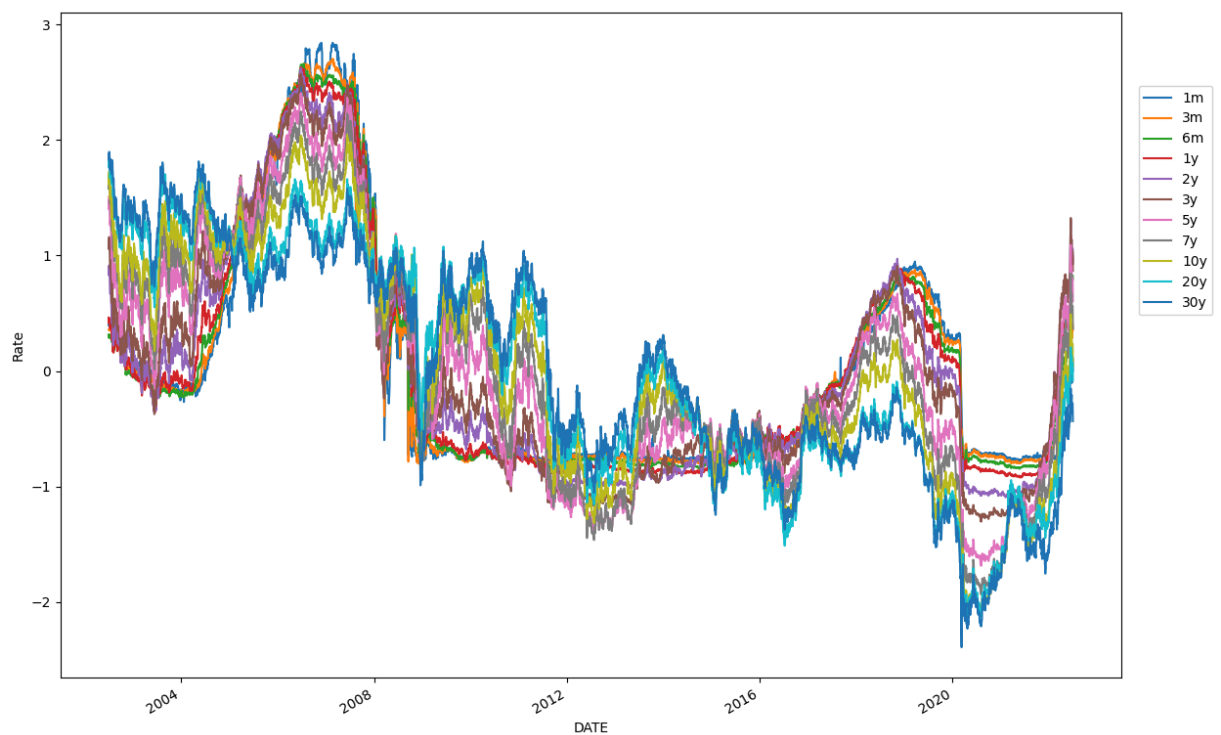
Fig. 11: Scaled Yield Curve Plot
