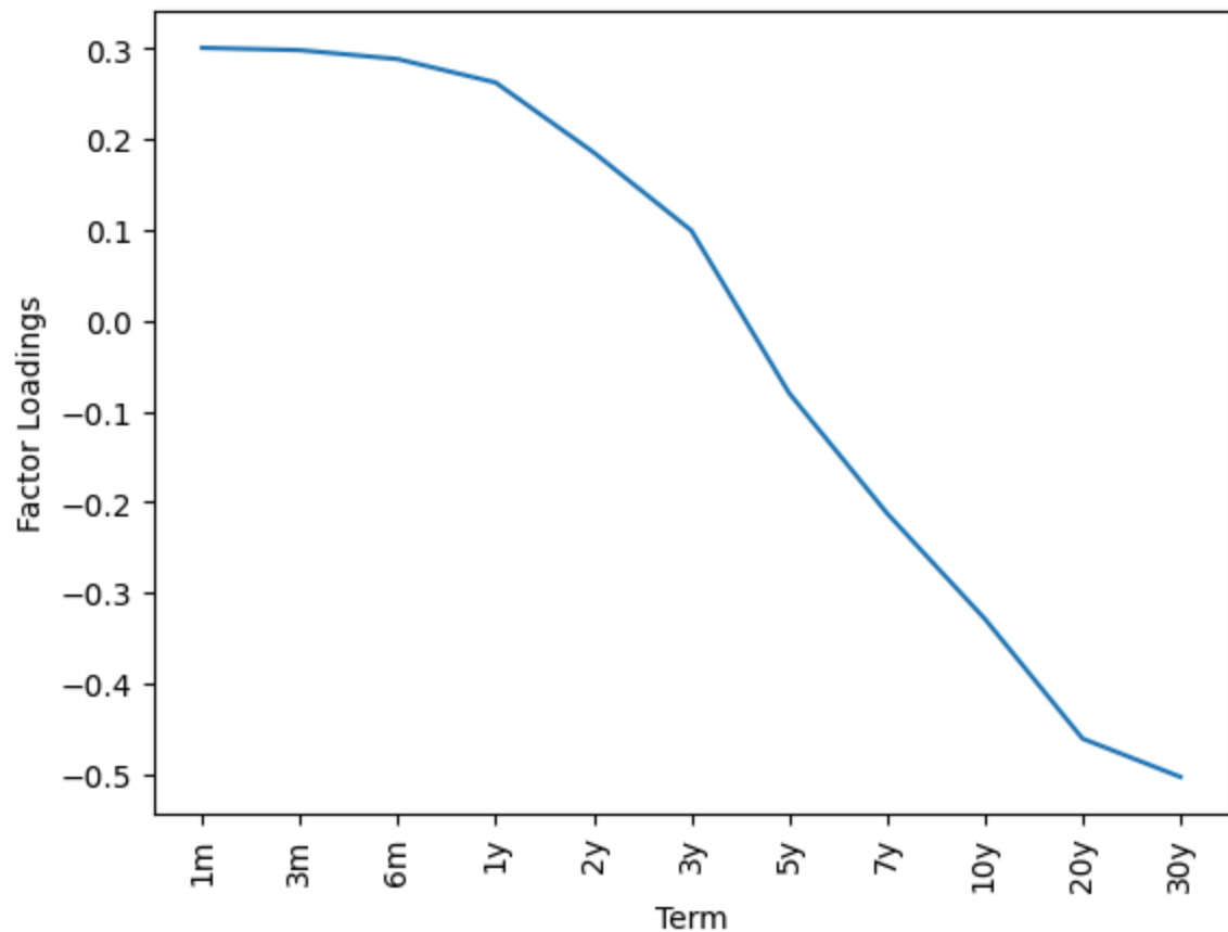
Fig. 3: The Second Factor Loading
